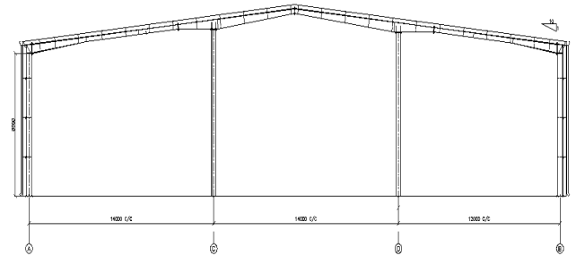
Fig. 2 Internal frame without crane
