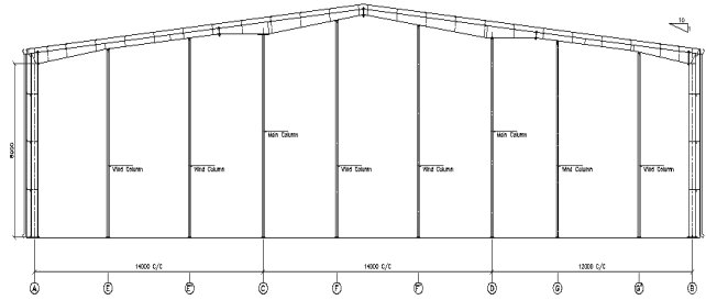
Fig. 1 End frame with wind columns
