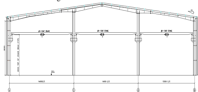
Fig. 3 Internal main frame with cranes
