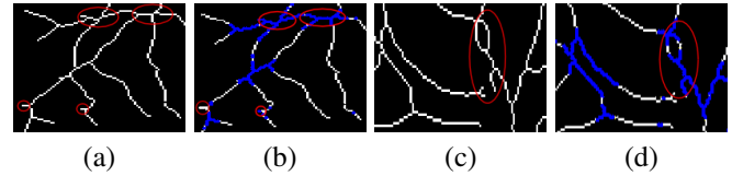
Fig. 2. Challenges in keypoint detection. Red ellipses point to artefacts due to segmentation and skeletonization. (a),(c) Skeletonized vessel maps; (b),(d) Keyoints detected with VKD.
