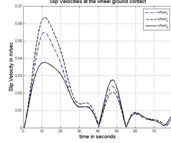
Fig. 10. L_2 norm of the slip velocities
