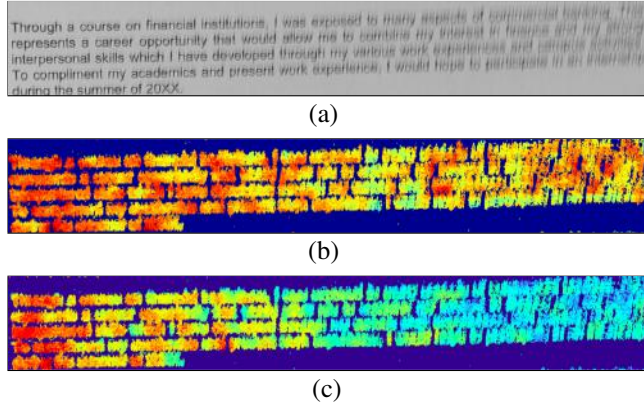
Fig. 3. Blur maps obtained using DCNN network and proposed pipeline. Red indicates a high score i.e. high quality while blue indicates a low score, i.e. low quality for a patch. Part (a) shows an image with both motion and focus blur. Part (b) shows the obtained blur map with DCNN network using OCR accuracies as ground truth. Part (c) shows the blur map generated using the pipeline and ground truth values proposed in this work.
